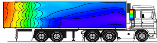
Doors open with BlueSeal air curtain
